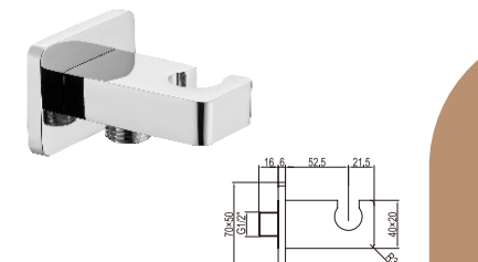
CZT072 Shower bracket (brass) Finish: chrome, with outlet
