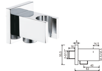
CZT002 Shower bracket (brass) Finish: chrome, with outlet
