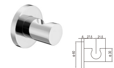
CZT044 Shower bracket (brass) Finish: chrome
