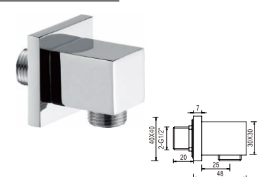
CZT007 Shower wall outlet (brass) Finish: chrome
