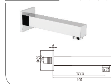
CST1029 Brass spout set Finish: chrome
