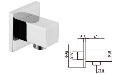
CZT067 Shower wall outlet (brass) Finish: chrome
