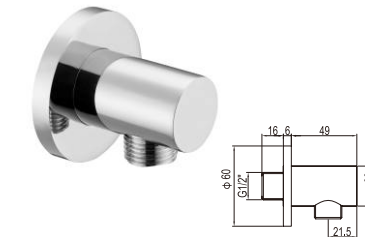
CZT043 Shower wall outlet (brass) Finish: chrome
