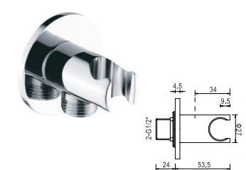
CZT003 Shower bracket (brass) Finish: chrome, with outlet
