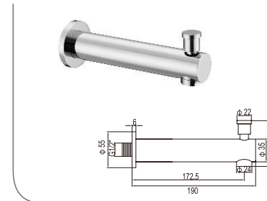
CST1027-1 Brass spout set Lift-up on/off Finish: chrome
