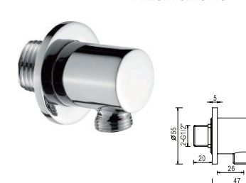
CZT008 Shower wall outlet (brass) Finish: chrome
