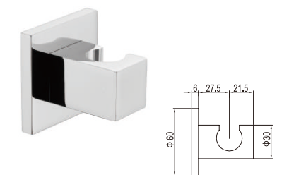
CZT068 Shower bracket (brass) Finish: chrome
