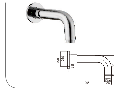
CST1023 Brass spout set Finish: chrome
