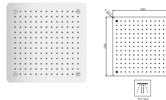
DPG5020JS 500mm square ceiling mounted rainfall shower head (SUS 304)
