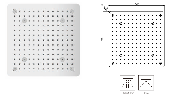
DPG5020JS-1 500mm square ceiling mounted rainfall shower head (SUS 304)
