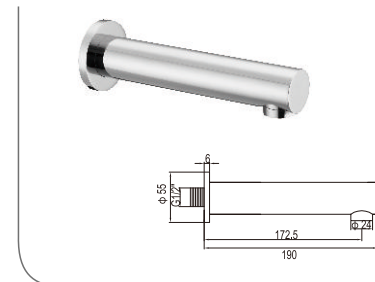
CST1027 Brass spout set Finish: chrome
