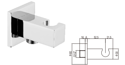
CZT066 Shower bracket (brass) Finish: chrome, with outlet
