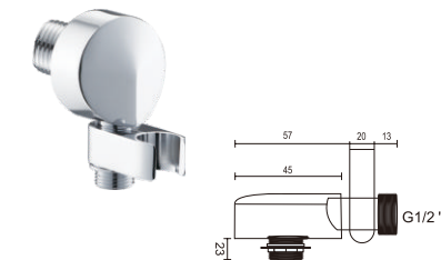
CZT022 Shower bracket (brass) Finish: chrome, with outlet
